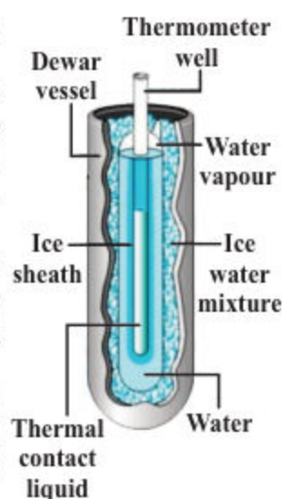
Figure 15.2 A triple point cell in which solid ice liquid water are water vapour co-exist in thermal equilibrium. The bulb of the constant volume gas thermometer is shown inserted into the well of the cell.
