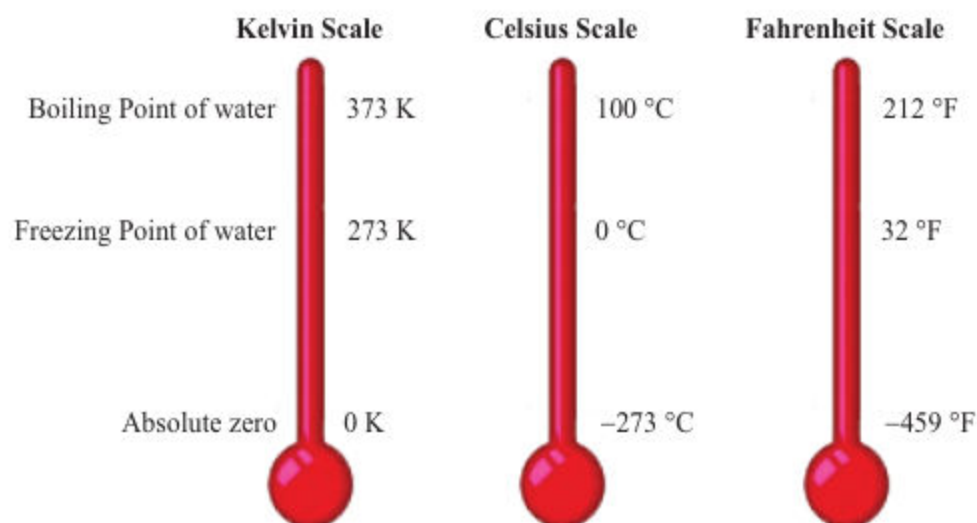
Figure 15.1 Scales of temperature mentioning the different temperatures.
