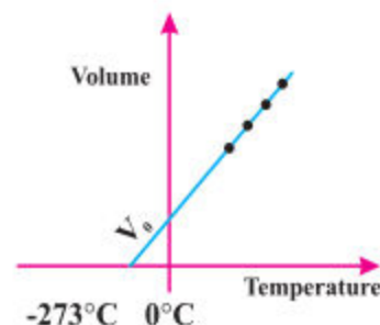
Figure 15.5 Shows relation between temperature and volume
